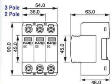
DC-SPD2P-1000V DC-SPD3P-1000V DC SURGE PROTECTIVE DEVICE 10-20 kA
