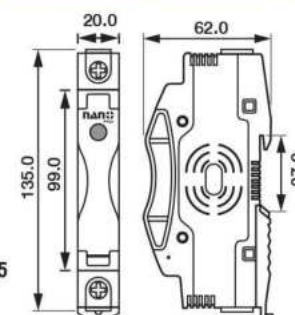
1P 1500V 10x85 DC-FH32-1500V DC HOLDER FUSE with LED
