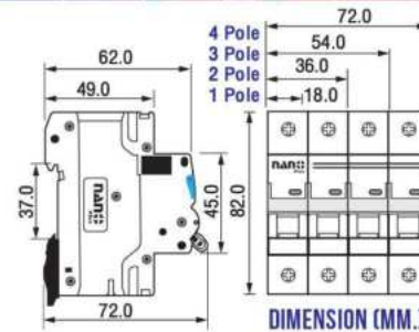
1 Pole 250VDC
