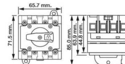
DC-ISW44C32 DC ISOLATING SWITCH
