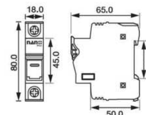
1P 1000V 10x38 DC-FH32-1000V DC HOLDER FUSE
