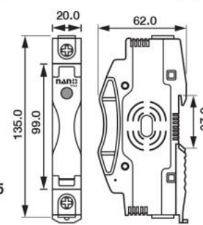
1P 1500V 10x85 DC-FH32-1500V DC HOLDER FUSE with LED
