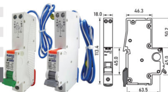
1 Pole 6 kA 30mA
