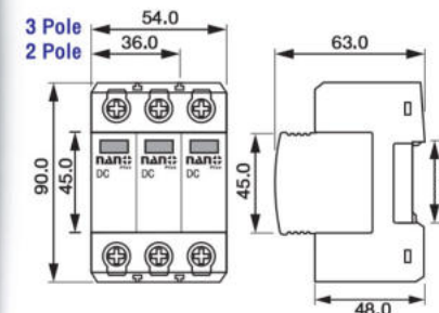
DC-SPD2P-1000V DC-SPD3P-1000V DC SURGE PROTECTIVE DEVICE 10-20 kA
