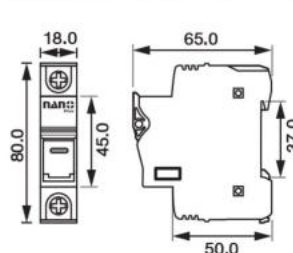
1P 1000V 10x38 DC-FH32-1000V DC HOLDER FUSE
