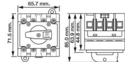
DC-ISW44C32 DC ISOLATING SWITCH
