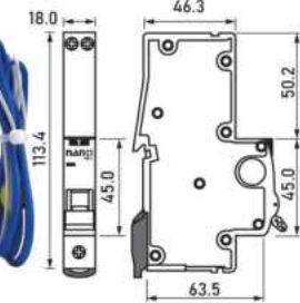
1 Pole 10kA 30mA
