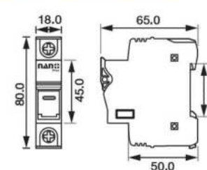
1P 1000V 10x38 DC-FH32-1000V DC HOLDER FUSE
