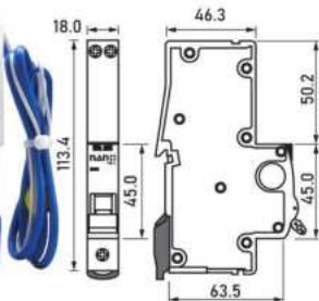
1 Pole 10kA 30mA
