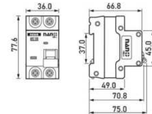
1 Pole 10kA 30mA
