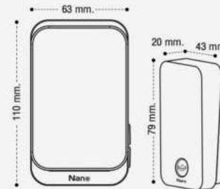
DOOR CHIME (INDOOR)
