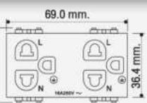
SC-PV601 / SC-PV602 SC-PV601B / SC-PV602B
